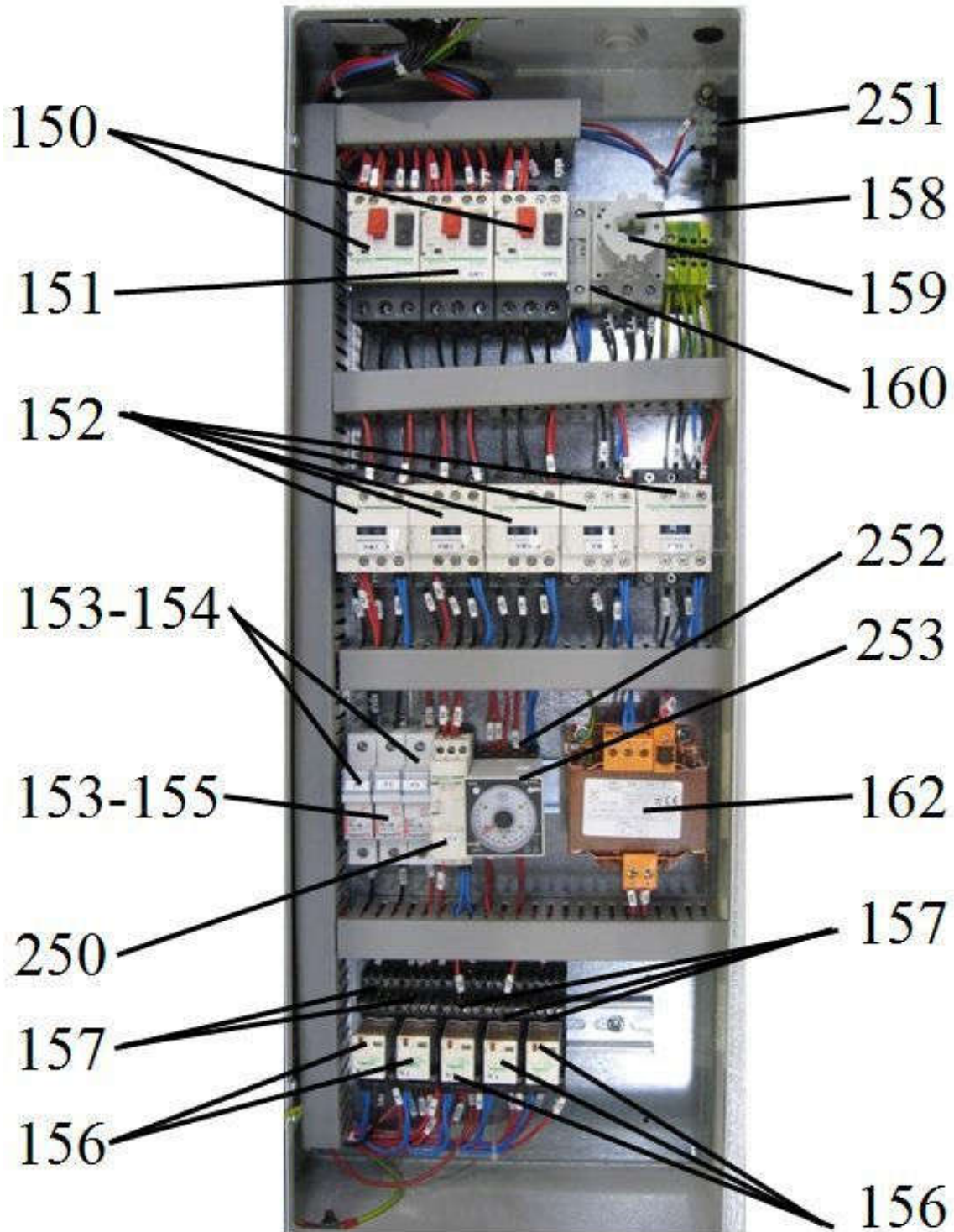
Fig 7 - Electric spare parts for combustion machine with electromechanical control panel -
