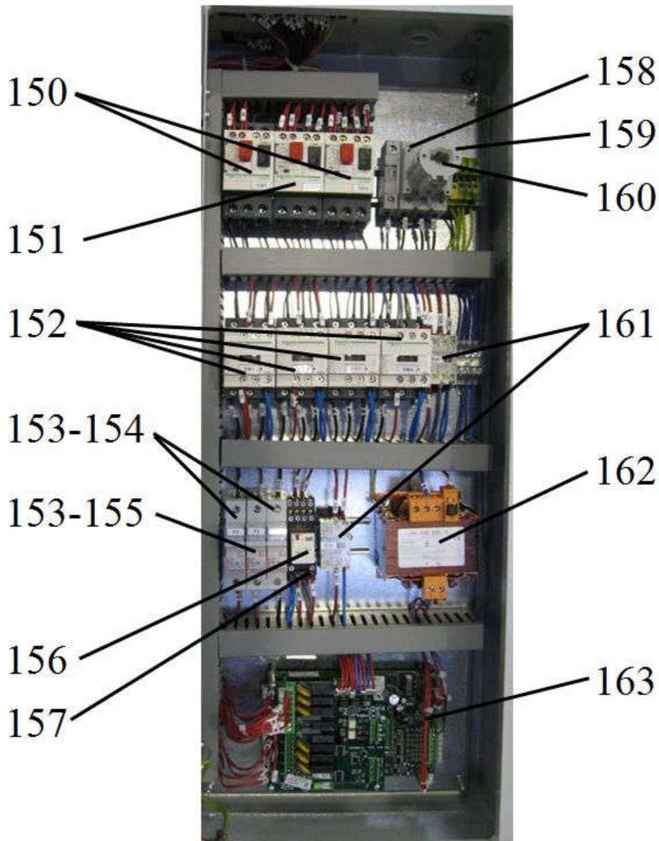
Fig 8 - Electric spare parts - combustion machine with electronic control panel -
