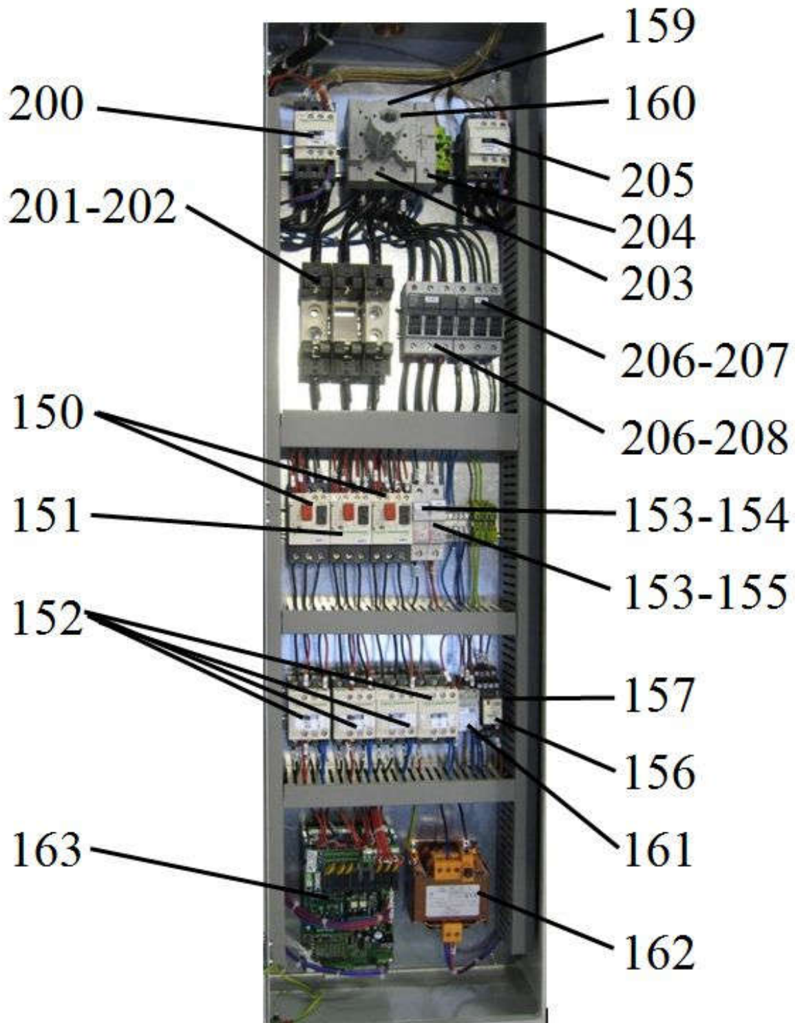
Fig 9 - Electric spare parts - electric machine with electronic control panel -
